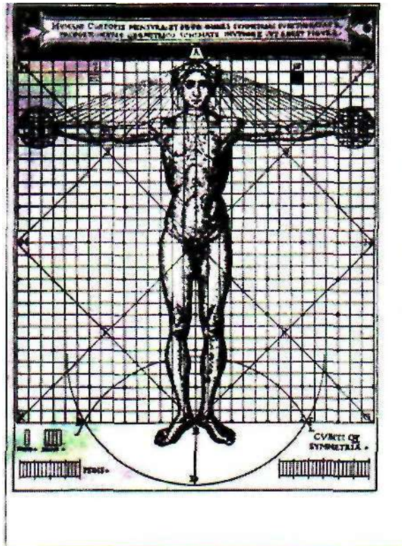
Fig. 9-25. Vitruvius' canon.
